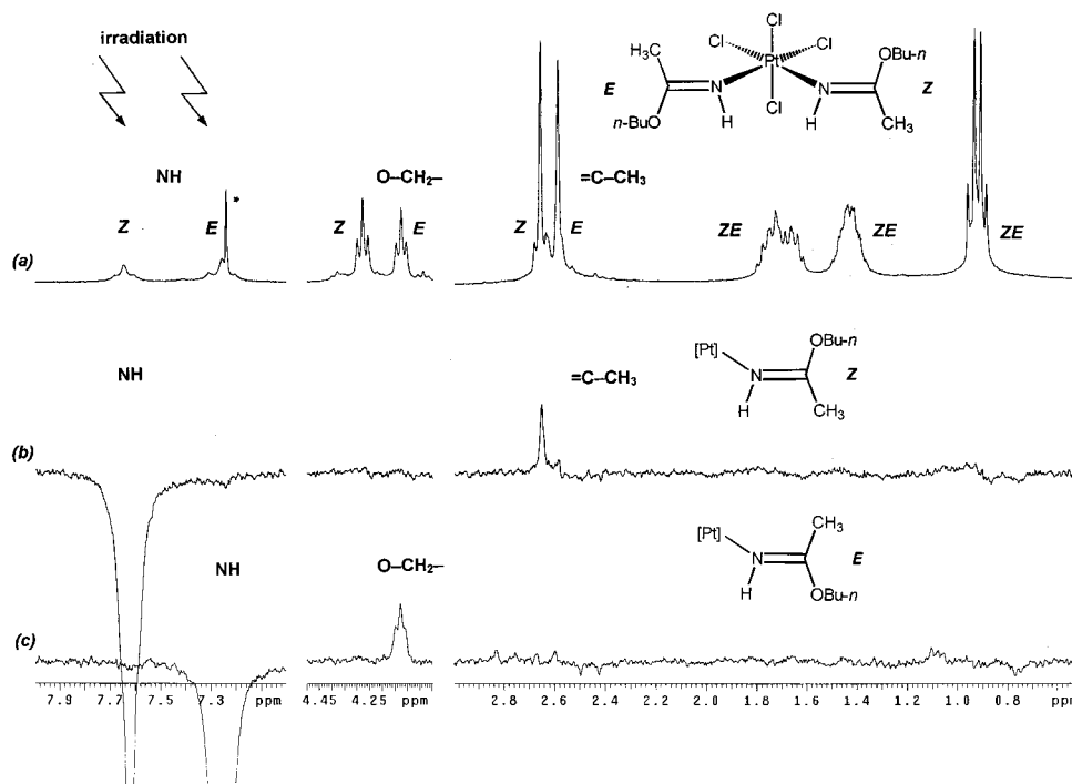
Figure 1. (a) 1 H NMR spectrum (in CDCl 3 ) of cis -[PtCl 4 {( E )-NH=C(Me)OBu- n }{( Z )-NH=C(Me)OBu- n }] (*): CHCl 3 . (b) NOE difference spectrum upon irradiation at the higher frequency NH ( Z configuration). (c) NOE difference spectrum upon irradiation at the lower frequency NH ( E configuration).
