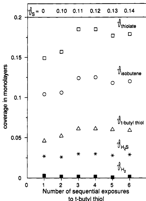
Figure 5. Amount of tert -butyl thiolate formed from tert -butyl thioalcohol adsorption and amounts of tert -butyl thioalcohol, \text{H}_2\text{S} , isobutene, and \text{H}_2 generated above 400 K from tert -butyl thiolate decomposition as a function of surface sulfur coverage on adsorption. Amounts quoted as fractions of a monolayer (1 ML = 8.54 \times 10^{14} molecules \text{cm}^{-2} ).
