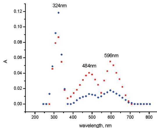
Figure 1. Calibrated 12 UV–vis spectra acquired 50 ns after LFP generation of PhCCl in TMB/pentane solution; blue spectrum at 0.26 mM TMB, red spectrum at 0.75 mM TMB.
