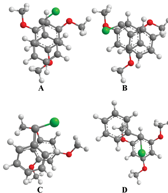
Figure 2. Four computed complexes formed between PhCCl and TMB (in perspective, carbene on top; green, chlorine; red, oxygen).
