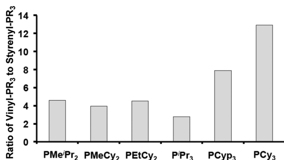
Figure 6. Ratio of the vinylphosphonium salt to the styrenylphosphonium salt for the different catalysts 1-R 3 (R 3 = Cy 3 , Cyp 3 , Pr 3 , EtCy 2 , EtPr 2 , MeCy 2 , MePr 2 ).
