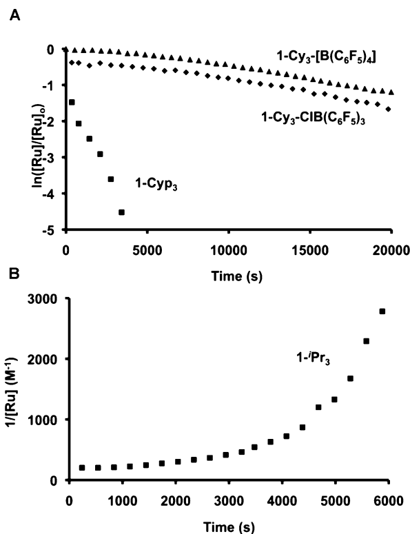
Figure 4. (A) Pseudo-first-order plots for the reactions of 1-Cy 3 and 1-Cyp 3 with o -isopropoxystyrene (1:30) at 243 K. (B) Second-order plot for the reaction of 1-iPr 3 and o -isopropoxystyrene (1:1) at 190 K.
