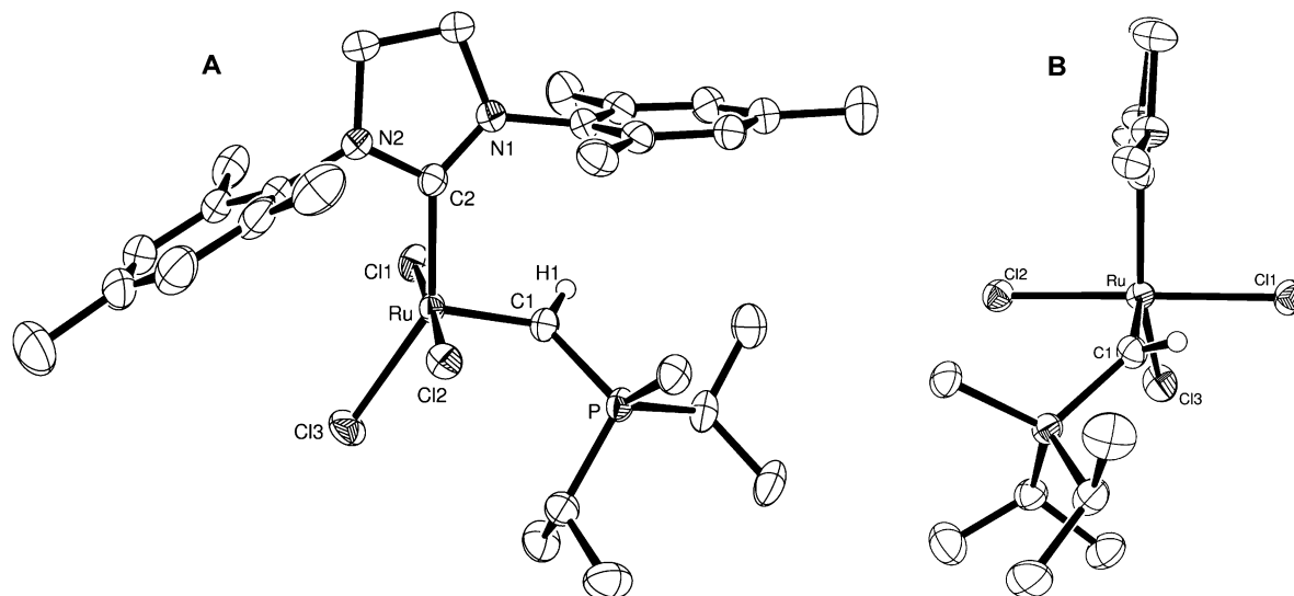
Figure 1. Crystal structure of 1-Me'Pr 2 -Cl : (A) front view; (B) side view. See Supporting Information for an ORTEP diagram of 1-MeCy 2 -Cl
