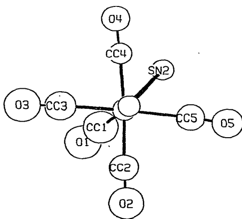
Fig. 2. View of the vanadium coordination sphere looking down the Sn(1)—V bond showing the C_{2v} symmetry of a monocapped trigonal prism.
