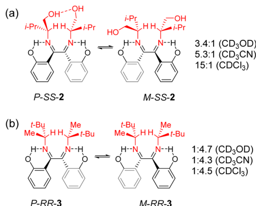
Scheme 1. Solvent Effects on the Stereoselectivity of Diimines Formed from (a) L-Valinol and (b) (R)-3,3-Dimethyl-2-butylamine
