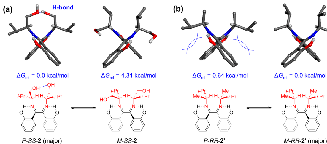
Figure 3. Calculated global energy minimum structures of (a) P -SS- 2 and M -SS- 2 as well as (b) P -RR- 2' and M -RR- 2' , an imine ( 2' ) formed between 1 and ( R )-3-methyl-2-butylamine.
