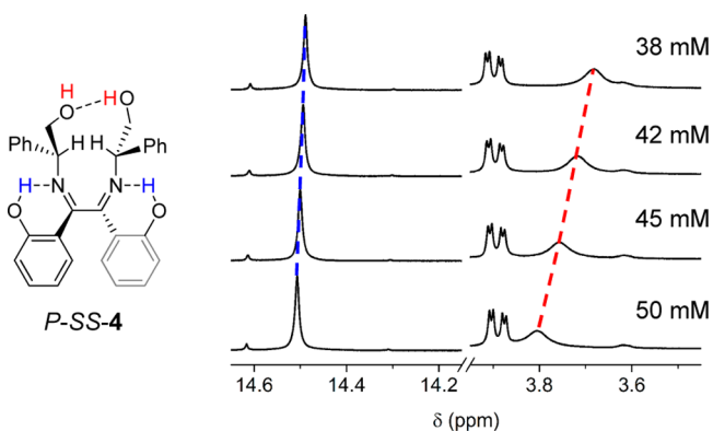
Figure 4. Concentration effect for the chemical shifts of the phenolic OH and the hydroxyl OH of SS-4 in \text{CDCl}_3 .
