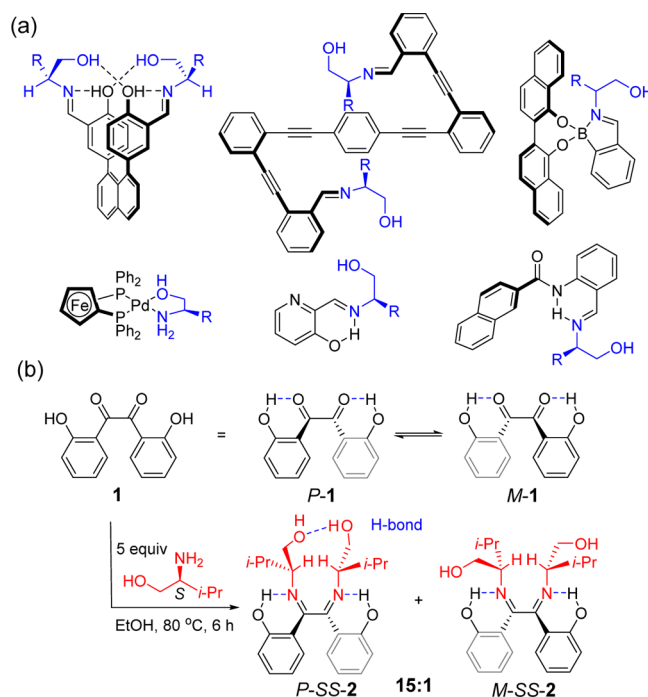
Figure 1. (a) Reported chiroptical probes and (b) 2,2'-dihydroxybenzil (1) for the chirality sensing of amino alcohols.
