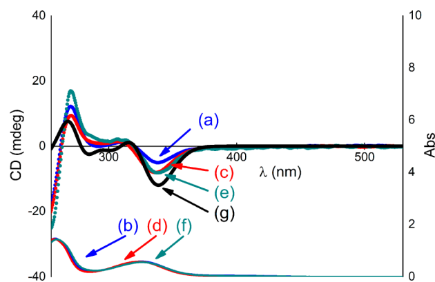
Figure 5. Measured CD spectrum and UV-vis spectrum (75 \mu\text{M} , 10 mm cell, at 20 ^\circ\text{C} ) of SS-2 in EtOH (a and b), \text{CH}_3\text{CN} (c and d), and \text{CHCl}_3 (e and f) and simulated CD spectrum of P-SS-2 (g).
