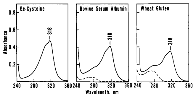
Figure 3. Absorption spectra of S-2-(2-quinolyethyl)-L-cysteine (Qe-cysteine), 2-vinylquinoline-modified whole wheat gluten (0.208 mg/ml), and BSA (0.082 mg/ml) in 0.1 N acetic acid (—) and of unmodified proteins at the same concentration (---)
