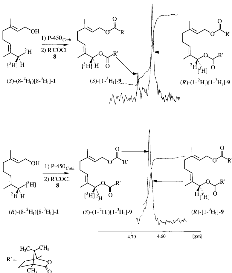
Fig. 2. 384-MHz ^1\text{H} -Decoupled ^3\text{H} -NMR spectra (in \text{CDCl}_3 ) of the derivatives of 8-hydroxygeraniol, obtained from enzymatic hydroxylation of geraniols with microsomal cytochrome P-450 Cath. . Chemical shifts are given in ppm ( \delta(\text{TMS}) = 0 ).
