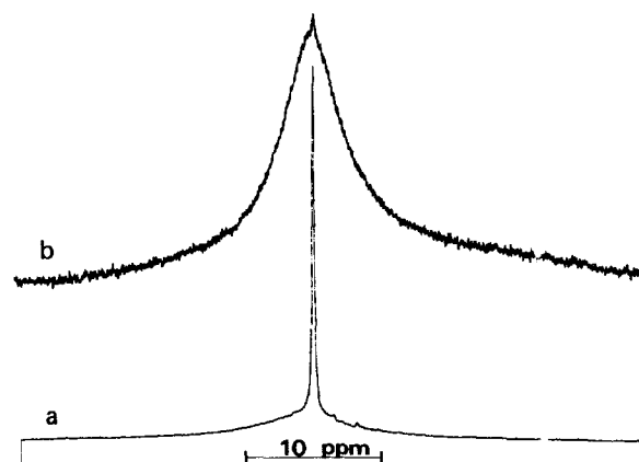
Fig. 4. The ^{27}\text{Al} NMR spectra of (a) 0.1 M \text{Al}^{3+} , 0.1 M \text{F}^- ; (b) 0.1 M \text{Al}^{3+} , 0.2 M \text{F}^- . Chemical shifts are relative to [\text{Al}(\text{H}_2\text{O})_6]^{3+} as an external standard.
