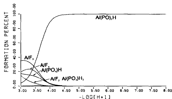
Fig. 3. Effect of pH upon the species distribution of a solution that is 10^{-7} M \text{Al}^{3+} , 1 mM \text{F}^- , 1 mM \text{PO}_4^{3-} , 1 mM ADP and 1 mM ATP.
