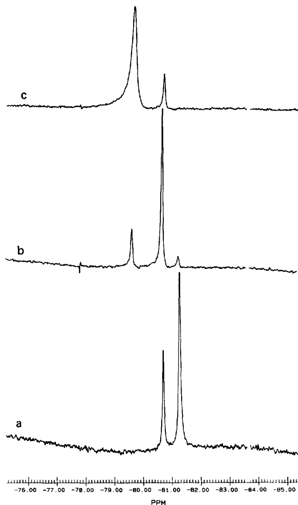
Fig. 5. The ^{19}\text{F} NMR spectra of (a) 50 mM \text{AlCl}_3 , 50 mM \text{NaF} ; (b) 33 mM \text{AlCl}_3 , 67 mM \text{NaF} ; (c) 25 mM \text{AlCl}_3 , 75 mM \text{NaF} . Chemical shifts are relative to \text{F}^- as an external standard.
