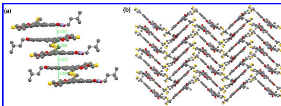
Figure 2. (a) Head to tail arrangement of molecule 8j , and (b) its herringbone-like packing viewed along the a axis.
