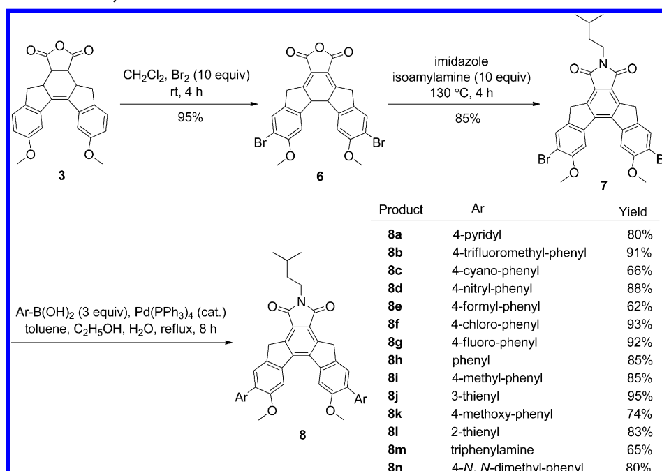
Scheme 2. Synthesis of Imide Dyes 8a–n
