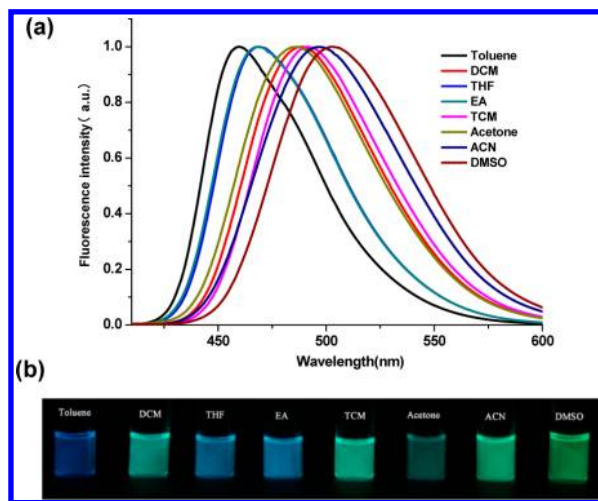
Figure 3. (a) Fluorescence spectra of 8h in different solvents ( 1 \times 10^{-5} M), and (b) images for the fluorescent colors of 8h in corresponding solution under ultraviolet light (365 nm).
