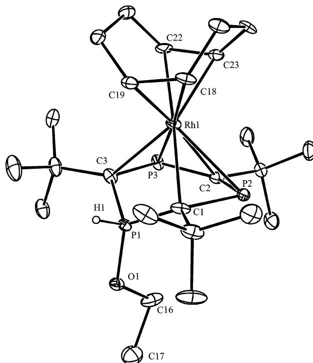
Figure 7. Thermal ellipsoid plot (25% probability surface) of the structure of the cationic component of [(\text{COD})\text{Rh}\{\eta^5-[(\text{H})(\text{EtO})\text{P}]\text{P}_2\text{C}_3\text{Bu}^t_3\}][\text{BAR}^f_4] ( 11 ); carbon bound hydrogen atoms are omitted for clarity. Rh(1)–C(1) 2.312(4), Rh(1)–C(3) 2.361(4), Rh(1)–C(2) 2.389(4), Rh(1)–P(3) 2.4898(14), Rh(1)–P(2) 2.520(1), P(1)–O(1) 1.579(5), P(1)–C(1) 1.628(5), P(1)–C(3) 1.801(5), P(2)–C(2) 1.781(5), P(2)–C(1) 1.857(6), P(3)–C(2) 1.752(5), P(3)–C(3) 1.753(4), O(1)–P(1)–C(1) 119.0(3), O(1)–P(1)–C(3) 116.2(2), C(1)–P(1)–C(3) 108.8(2), C(2)–P(2)–C(1) 99.9(2), C(2)–P(3)–C(3) 108.0(2), P(1)–C(1)–P(2) 125.1(3), P(3)–C(2)–P(2) 135.8(3), P(3)–C(3)–P(1) 117.4(3).
