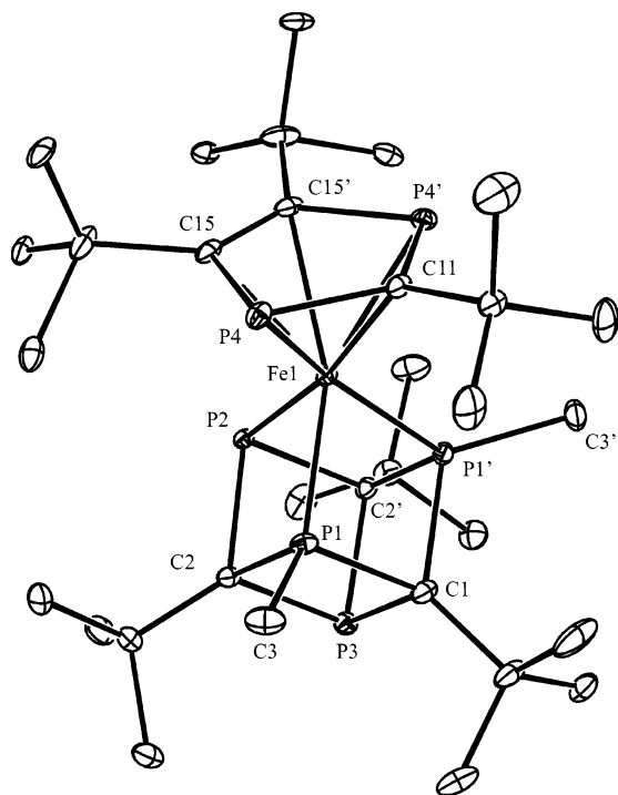
Figure 1. Thermal ellipsoid plot (25% probability surface) of the molecular structure of [(\eta^5\text{-}1,3\text{-P}_2\text{C}_3\text{Bu}_t^3)\text{Fe}\{\text{P}_2(\text{PMe})_2(\text{CBu}_t^3)\}] ( 4 ); hydrogen atoms are omitted for clarity. Fe(1)–P(1) 2.1570(10), Fe(1)–P(2) 2.3013(13), Fe(1)–P(4) 2.3287(10), Fe(1)–C(11) 2.254(5), Fe(1)–C(15) 2.217(3), P(4)–C(11) 1.742(3), P(4)–C(15) 1.796(4), P(1)–C(3) 1.837(4), P(1)–C(2) 1.855(3), P(1)–C(1) 1.890(4), P(2)–C(2) 1.937(3), P(3)–C(1) 1.881(5), P(3)–C(2) 1.902(4), P(1)–Fe(1)–P(1') 74.53(5), P(1)–Fe(1)–P(2) 74.38(4), C(2)–P(1)–C(1) 87.23(19), C(2)–P(1)–Fe(1) 100.99(11), C(1)–P(1)–Fe(1) 98.54(11), C(2)–P(2)–C(2') 85.1(2), C(2)–P(2)–Fe(1) 93.69(11), C(1)–P(3)–C(2) 86.15(15), C(2)–P(3)–C(2') 87.0(2), P(3)–C(1)–P(1) 93.08(19), P(1)–C(1)–P(1') 87.4(2), P(1)–C(2)–P(3) 93.54(16), P(1)–C(2)–P(2) 90.65(15), P(3)–C(2)–P(2) 93.78(16). Symmetry transformation used to generate equivalent atoms ' : x, -y+1/2, z .
