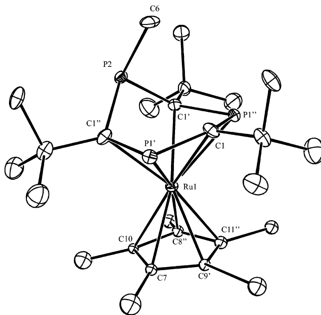
Figure 3. Thermal ellipsoid plot (25% probability surface) of the molecular structure of [\text{Cp}^*\text{Ru}(\eta^5\text{-(MeP)}_2\text{C}_3\text{Bu}_3)] ( 7 ); hydrogen atoms are omitted for clarity. Ru(1)–C(1) 2.328(14), Ru(1)–P(1') 2.448(10), C(1)–P(1') 1.802(5), C(1)–P(1'') 1.781(5), P(2)–C(1') 1.829(6), P(2)–C(1'') 1.841(6), P(1')–C(1)–P(1'') 116.4(3), C(1)–P(1')–C(2') 99.6(3), C(1')–P(2)–C(1'') 96.4(3). Symmetry transformations used to generate equivalent atoms: ' : y, z, x ; '' : z, x, y .
