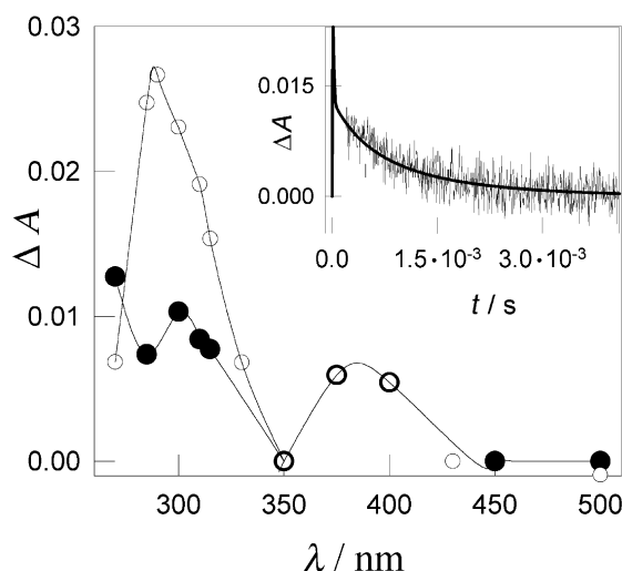
Fig. 3. Transient absorption spectra obtained at 400 \mu s after the flash irradiation of 9.2 \cdot 10^{-4} M K_4P_2O_8 solutions containing 5.6 \cdot 10^{-5} M toluene at pH 4: air-saturated (●) and N_2 -saturated (○). Inset: Experimental and simulated (solid line) absorbance profile obtained at 310 nm with 2.36 \cdot 10^{-3} M K_4P_2O_8 air-saturated solution at pH 4 containing 4.8 \cdot 10^{-3} M benzene.
