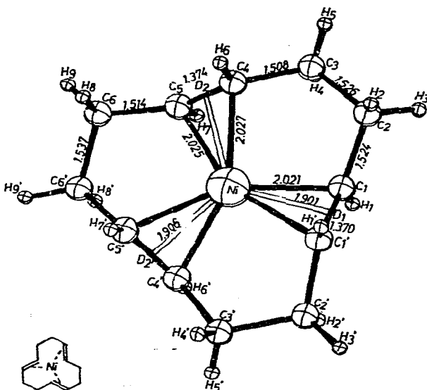
Fig. 1. A perspective drawing of all- trans -1,5,9-cyclododecatrien nickel. The standard deviations of the individual bond lengths are: C-C 0.007 Å; Ni-C 0.004 Å.
