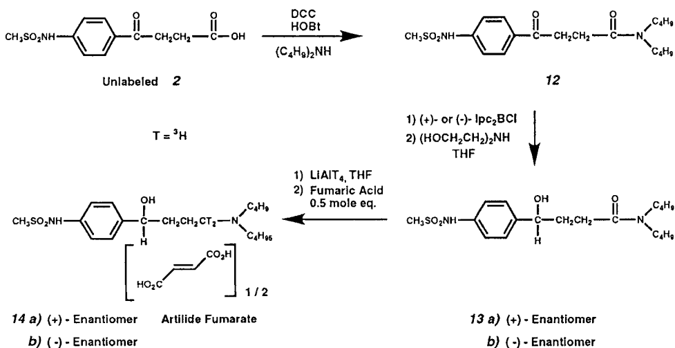
SCHEME 4.
