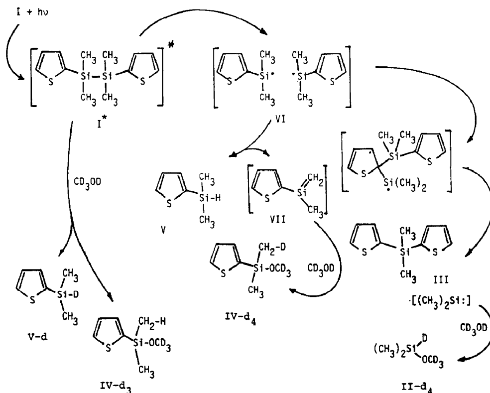
Scheme 2. Photochemical pathways of 1,1,2,2-tetramethyl-1,2-bis-(2'-thienyl)tetramethyldisilane.
