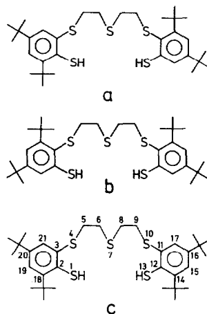
Fig. 2. Isomers of ^t\text{bu}_4\text{-dpttd-H}_2 .
