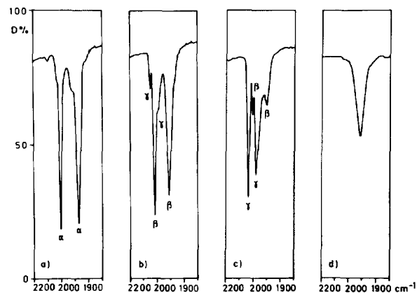
Fig. 1. IR monitoring of reaction (2) and (3) ( \nu(\text{CO}) region). (a) [\text{Ru}(\text{CO})_2(\text{S}_2\text{C}_6\text{H}_4)_2]^{2-} \rightleftharpoons \alpha ; (b) 1.5 h after addition of \text{S}(\text{C}_2\text{H}_4\text{Br})_2 at 20^{\circ}\text{C} ( [\text{Ru}(\text{CO})_2(\text{S}_2\text{C}_6\text{H}_4)(\text{C}_6\text{H}_4\text{S}_2\text{C}_2\text{H}_4\text{SC}_2\text{H}_4\text{Br})] \rightleftharpoons \beta ; [\text{Ru}(\text{CO})_2(\text{dpttd})] \rightleftharpoons \gamma ); (c) \sim 30 days after addition of \text{S}(\text{C}_2\text{H}_4\text{Br})_2 ; (d) [\text{Ru}(\text{CO})\text{dpttd}] in DMF (obtained according to eqn. (4)).
