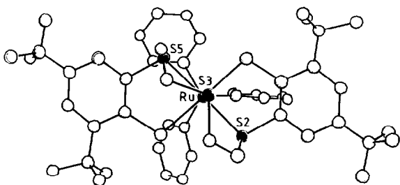
Fig. 7. View of [\text{Ru}(\text{PPh}_3)(^t\text{Bu}_4\text{-dpttd})] down the \text{SRuP} axis (H atoms omitted).
