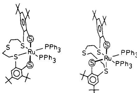
Fig. 4. Isomers of [\text{Ru}(\text{PPh}_3)_2(^t\text{bu}_4\text{-dpttd})] with trans and cis thiolato S atoms.
