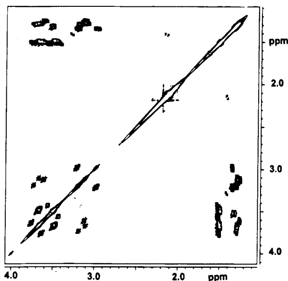
Figure 2. 2-D ^1\text{H} NMR spectrum of the mixture of the isomers of 7 .
