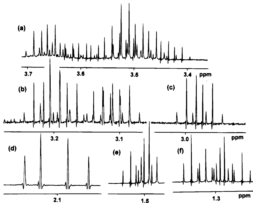
Figure 1. 500 MHz ^1\text{H} NMR spectrum of a mixture of the isomers of 7 . Key: (a–c) methylene proton resonances; (e, f) methyl resonances of ethyl groups; (d) \text{Cp}^* methyl resonances.
