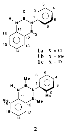
Fig. 1. Boron–nitrogen heterocycles derived from diazadiboranaphthalene.
