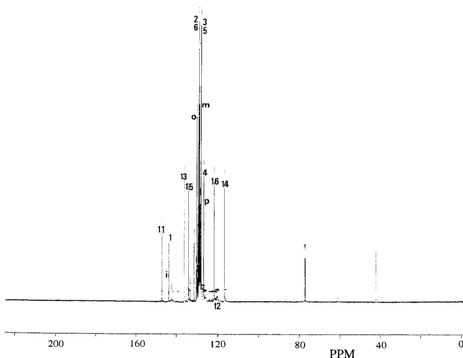
Fig. 2. ^{13}\text{C} NMR spectrum of the mixture containing 1a with (\text{C}_6\text{H}_5\text{NBCl})_3 : \delta ^{13}\text{C} (ppm) = 143.86(i), 129.63(o or m), 128.41(m or o) and 126.35(p). For the former compound, see text. Additional peaks near 40 and 60 ppm correspond to small amounts of \text{BDMA} \cdot \text{BCl}_3 and \text{BDMA} \cdot \text{HCl} . Solvent \text{CDCl}_3 , NS = 539, AQ = 1.769, SW = 18518.519.
