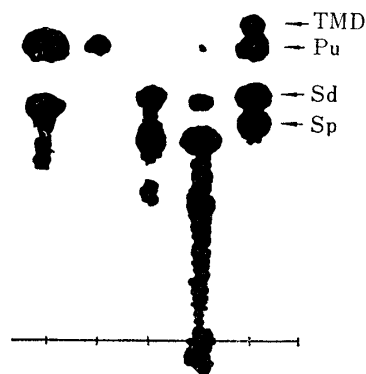
Fig. 10. Paper Electrophoresis of the Fraction separated by Amberlite XE-64
