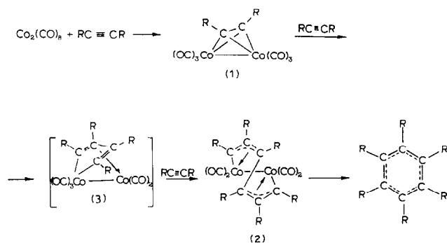
Fig. 1. Proposed mechanism of formation of symmetrically and asymmetrically substituted benzenes, showing the structures and role of complexes 1 , 2 and 3 .
