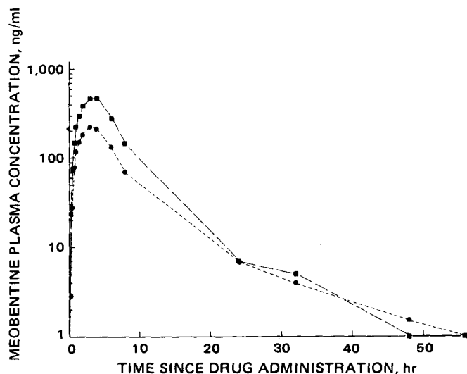
Figure 3 —Mean plasma mebentine concentrations (expressed as free base) following oral administration to normal human volunteers. Key: ●, 2.5 mg/kg ( n = 6 ); ■, 5.0 mg/kg ( n = 5 ).
