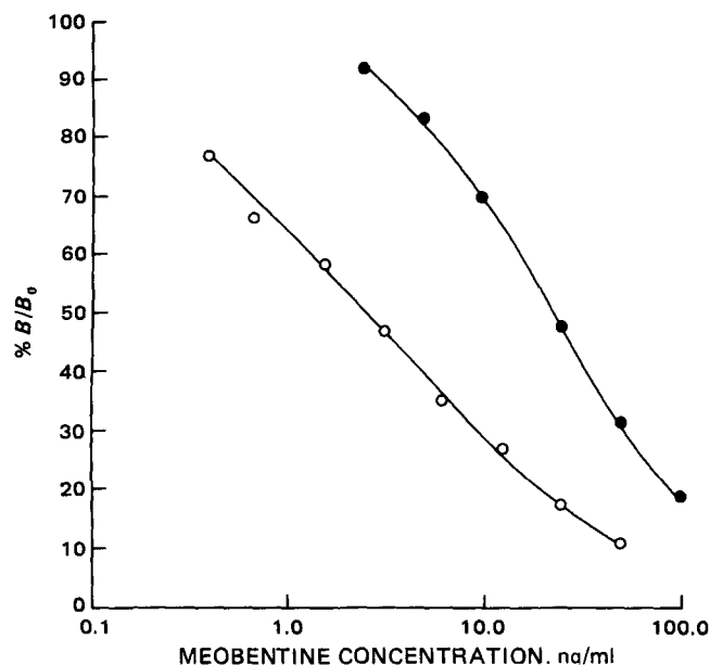
Figure 2 —Meobentine standard curves for tritium and radioiodine radioimmunoassays: mean of 8 curves in each case. Key: ●, [³H]meobentine; ○, [¹²⁵I]iodomeobentine.
