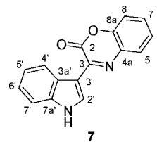
Figure 2. Structure of 3-(1 H -indol-3-yl)-2 H -1,4-benzoxazin-2-one ( 7 ).
