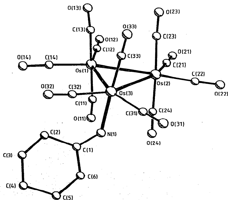
Fig. 1. The molecular structure of Os 3 (CO) 11 [NHC(CH 2 ) 5 ], the hydrogen atoms have been omitted for clarity.
