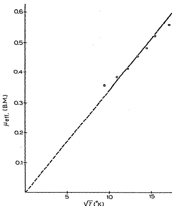
Fig. 4. Plot of \mu_{\text{eff}} vs. \sqrt{T} for the iodo derivative [\text{CoSaEn}]\text{I} (XIII).
