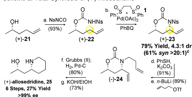
Scheme 2. Total Synthesis of (+)-Allosedridine a
