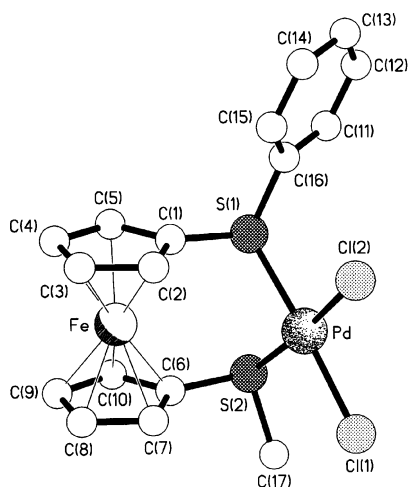
Figure 7. The molecular structure of 9 .
