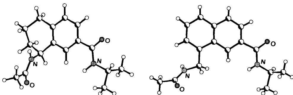
Fig. 3. PLUTO drawings of mimic derivatives 1c (left) and 3d (right). Crystal data and atomic parameters were submitted to the Cambridge Crystallographic Data Center.
