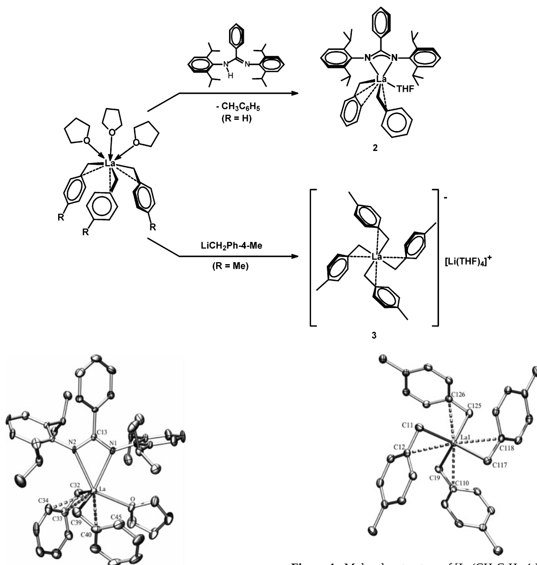
Figure 3. Molecular structure of [\text{PhC}(\text{NAr})_2]\text{La}(\text{CH}_2\text{Ph})_2(\text{THF}) ( 2 ), with 50% probability ellipsoids. Selected interatomic distances (Å) and angles (deg): \text{La}-\text{C}(32) = 2.590(5) , \text{La}-\text{C}(33) = 2.897(5) , \text{La}-\text{C}(34) = 3.030(3) , \text{La}-\text{C}(38) = 3.813(2) , \text{La}-\text{C}(39) = 2.632(3) , \text{La}-\text{C}(40) = 2.847(5) , \text{La}-\text{C}(45) = 3.401(5) , \text{La}-\text{N}(1) = 2.497(3) , \text{La}-\text{N}(2) = 2.581(3) , \text{La}-\text{O}(1) = 2.557(3) ; \text{La}-\text{C}(32)-\text{C}(33) = 87.0(3) , \text{La}-\text{C}(39)-\text{C}(40) = 83.3(2) .
