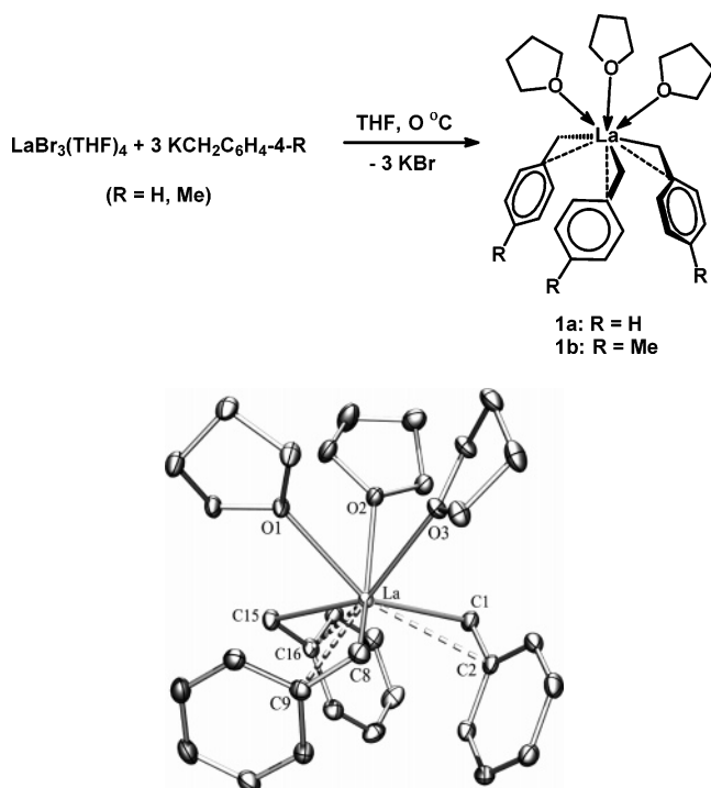
Figure 1. Molecular structure of [\text{La}(\text{CH}_2\text{Ph})_3(\text{THF})_3] ( 1a ), with 50% probability ellipsoids. Selected interatomic distances (Å) and angles (deg): La–C(1) = 2.648(2), La–C(2) = 2.968(2), La–C(8) = 2.649(2), La–C(9) = 2.972(2), La–C(15) = 2.639(2), La–C(16) = 2.994(2), La–O(1) = 2.6779(16), La–O(2) = 2.6630(15), La–O(3) = 2.6497(16); La–C(1)–C(2) = 88.05(13), La–C(8)–C(9) = 88.09(13), La–C(15)–C(16) = 89.53(14), O(1)–La–O(2) = 72.90(5), O(1)–La–O(3) = 74.59(5), O(2)–La–O(3) = 74.06(5).
