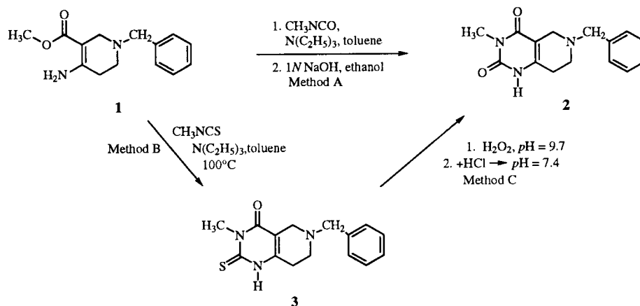
Scheme I
