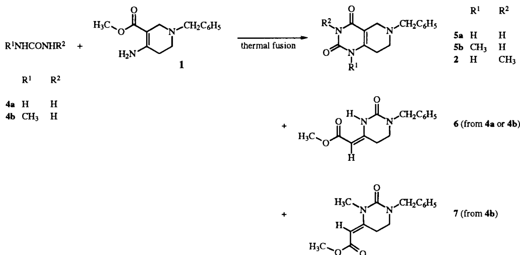
Scheme III
