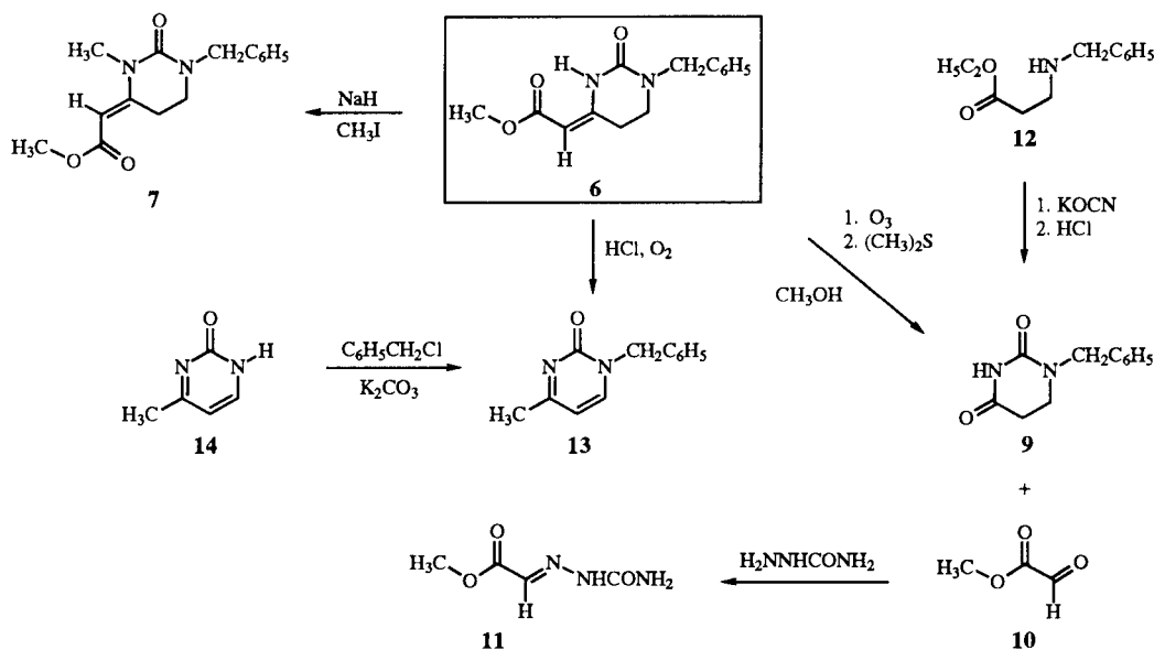
Scheme III
