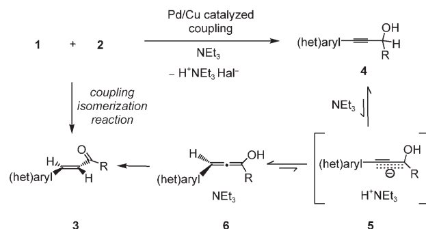
Scheme 2. Mechanistic rationale of the CIR.
