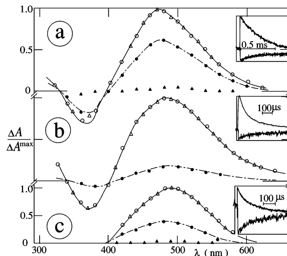
Figure 4. Transient absorption spectra of (a) Zn-I, (b) L_{II} , and (c) L_I in acetonitrile at 20 ns (○), 1 μs (△), 0.1 ms (●), and 1 ms (▲) after the 308 nm pulse. Insets: decay at 480 nm (upper) and 370 nm (lower).
