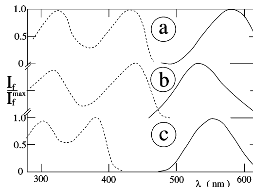
Figure 2. Fluorescence emission (right, \lambda_{\text{exc}} = 380 nm) and excitation (left, \lambda_{\text{em}} = 550 nm) spectra of (a) Zn-II, (b) Zn-I, and (c) \text{L}_\text{I} in MCH at 25 °C.
