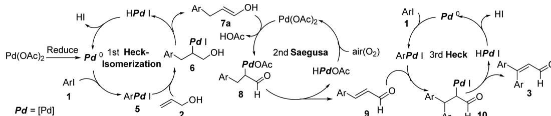
Scheme 1. Possible Mechanism for the Domino Heck-Isomerization/Saegusa/Heck Reaction
