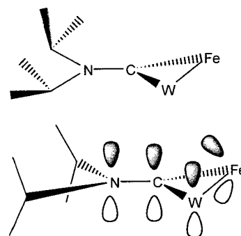
Figure 3. Orientational possibilities for the bridging aminomethylidyne ligand in 8 .
