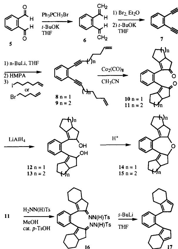
Scheme 1. Synthesis of bis(cyclopentadiene) 17 .
