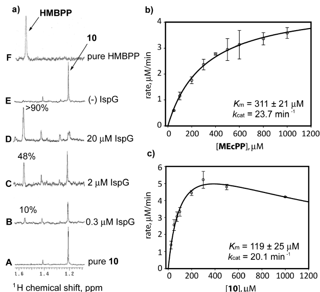
Figure 1. (a) ^1\text{H} NMR analysis of the IspG-catalyzed conversion of 10 to HMBPP. Reaction conditions: 100 mM Tris buffer (pH 8.0) at 37 °C for 30 min with 5 mM dithionite, 1 mM MV, 1 mM 10 , and various IspG concentrations. (b) Michaelis–Menten analysis of MEcPP ( 6 ). (c) Michaelis–Menten analysis of 10 .
