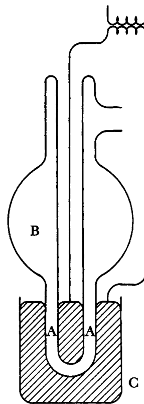
Fig. 1.—Discharge chamber.
