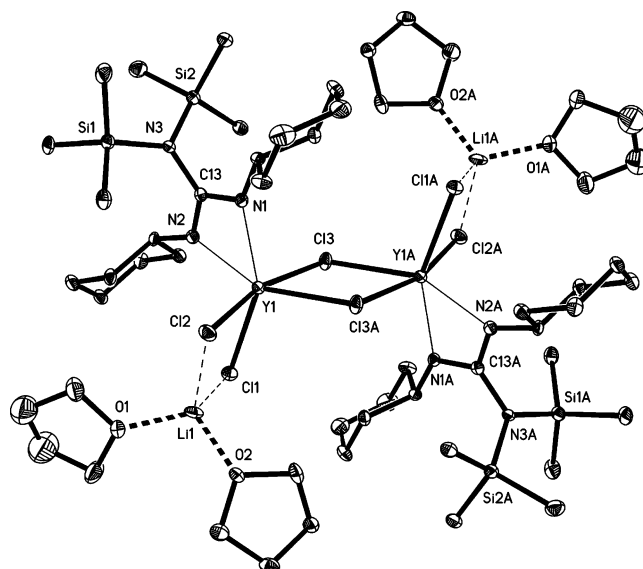
Figure 1. ORTEP diagram (30% probability thermal ellipsoids) of \{[(\text{Me}_3\text{Si})_2\text{NC}(\text{NCy})_2]\text{Y}\{(\mu\text{-Cl})_2\text{Li}(\text{THF})_2(\mu\text{-Cl})\}_2\} ( 1 ) showing the non-hydrogen and non-carbon (except C(13)) atom numbering scheme. Hydrogen atoms are omitted for clarity. Selected bond distances [Å] and angles [deg]: \text{Y}(1)\text{--}\text{N}(2) 2.298(4), \text{Y}(1)\text{--}\text{N}(1) 2.304(5), \text{Y}(1)\text{--}\text{Cl}(2) 2.6227(16), \text{Y}(1)\text{--}\text{Cl}(1) 2.6385(16), \text{Y}(1)\text{--}\text{Cl}(3) 2.7023(15), \text{Y}(1)\text{--}\text{Cl}(3\text{A}) 2.7065(15), \text{Y}(1)\text{--}\text{C}(13) 2.738(6), \text{Y}(1)\text{--}\text{Li}(1) 3.540(10), \text{Cl}(1)\text{--}\text{Li}(1) 2.415(11), \text{Cl}(2)\text{--}\text{Li}(1) 2.344(10), \text{Cl}(3)\text{--}\text{Y}(1\text{A}) 2.7065(15), \text{Li}(1)\text{--}\text{O}(2) 1.891(11), \text{N}(1)\text{--}\text{C}(13) 1.333(7), \text{N}(3)\text{--}\text{C}(13) 1.438(7), \text{N}(2)\text{--}\text{C}(13) 1.320(7), \text{N}(2)\text{--}\text{Y}(1)\text{--}\text{N}(1) 57.76(16), \text{Cl}(2)\text{--}\text{Y}(1)\text{--}\text{Cl}(1) 84.23(5), \text{Cl}(3)\text{--}\text{Y}(1)\text{--}\text{Cl}(3\text{A}) 78.02(5).
