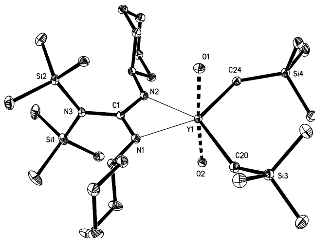
Figure 2. ORTEP diagram (30% probability thermal ellipsoids) of \{(\text{Me}_2\text{Si})_2\text{NC}(\text{NCy})_2\}\text{Y}(\text{CH}_2\text{SiMe}_3)_2(\text{THF})_2 ( 2 ) showing the non-hydrogen and non-carbon (except C(1), C(20), and C(24)) atom numbering scheme. Hydrogen atoms and carbon atoms of THF are omitted for clarity. Selected bond distances [Å] and angles [deg]: Y(1)–C(20) 2.462(2), Y(1)–C(24) 2.473(2), Y(1)–N(1) 2.4165(17), Y(1)–N(2) 2.3833(17), Y(1)–O(1) 2.3777(14), Y(1)–O(2) 2.4029(14), Y(1)–C(1) 2.838(2), N(1)–C(1) 1.337(3), C(1)–N(2) 1.328(3), C(20)–Y(1)–C(24) 112.40(7) , N(2)–Y(1)–N(1) 55.80(6) , O(1)–Y(1)–O(2) 174.50(5) .
