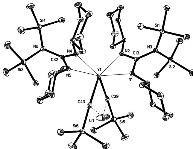
Figure 4. ORTEP diagram (30% probability thermal ellipsoids) of \{(Me_3Si)_2NC(Cy)_2\}_2Y(\mu-CH_2SiMe_3)_2Li ( 6 ) showing the non-hydrogen and non-carbon (except C(13), C(32), C(39), and C(43)) atom numbering scheme. Hydrogen atoms are omitted for clarity. Selected bond distances [Å] and angles [deg]: Y(1)-N(2) 2.3497(14), Y(1)-N(4) 2.3626(15), Y(1)-N(5) 2.3914(13), Y(1)-N(1) 2.3998(14), Y(1)-C(39) 2.543(2), Y(1)-C(43) 2.5460(17), Y(1)-C(13) 2.8118(18), Y(1)-C(32) 2.8167(17), Y(1)-Li(1) 2.882(4), Li(1)-C(43) 2.083(5), Li(1)-C(39) 2.103(5), Li(1)-C(41) 2.514(5), Li(1)-C(45) 2.947(5), Li(1)-C(42) 3.551(5), Li(1)-C(44) 3.482(5), N(1)-C(13) 1.336(2), N(2)-C(13) 1.3274(19), N(4)-C(32) 1.332(2), N(5)-C(32) 1.334(3), N(4)-Y(1)-N(5) 56.25(5), N(2)-Y(1)-N(1) 56.33(4), C(39)-Y(1)-C(43) 88.95(6), C(39)-Li(1)-C(43) 116.78(4), C(39)-Si(5)-C(42) 110.99(9), C(39)-Si(5)-C(41) 108.91(10), C(39)-Si(5)-C(40) 114.59(9), C(43)-Si(6)-C(44) 110.67(9), C(43)-Si(6)-C(45) 109.39(10), C(43)-Si(6)-C(46) 114.82(10).
