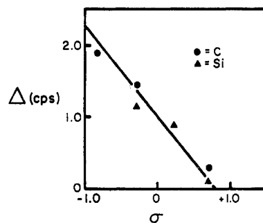
Figure 3.—Correlation of N(CH 3 ) 2 shift with Hammett's \sigma constants.
