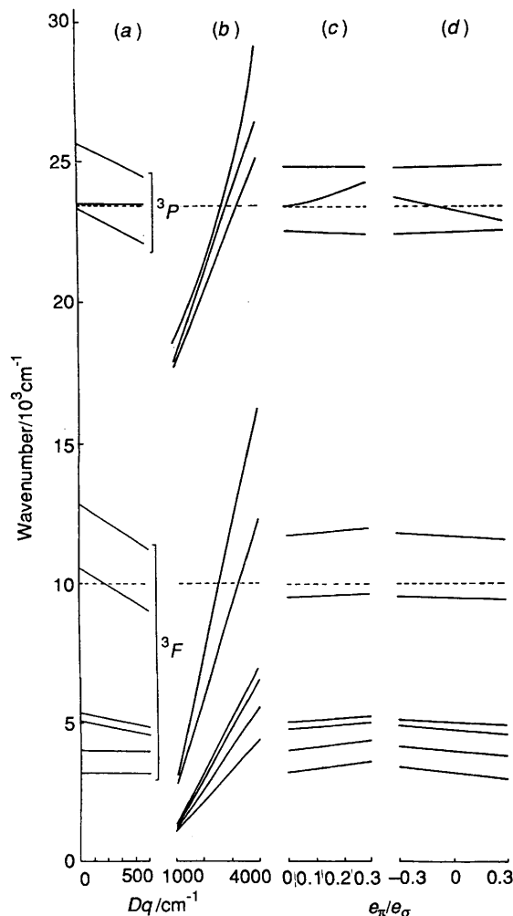
Figure 5. Computed electronic transitions for [\text{NiL}(\text{I})]_2[\text{As}_6\text{I}_8] . The effects of varying: (a) Dq^{\text{I}} with Dq^{\text{P}} = 3000 \text{ cm}^{-1} , e_{\pi}^{\text{P}}/e_{\sigma}^{\text{P}} = 0.15 , e_{\pi}^{\text{I}} = 0.0 \text{ cm}^{-1} ; (b) Dq^{\text{P}} with Dq^{\text{I}} = 350 \text{ cm}^{-1} , e_{\pi}^{\text{I}}/e_{\sigma}^{\text{I}} = 0.10 , e_{\pi}^{\text{P}}/e_{\sigma}^{\text{P}} = 0.15 ; (c) e_{\pi}^{\text{I}}/e_{\sigma}^{\text{I}} with Dq^{\text{I}} = 350 \text{ cm}^{-1} , Dq^{\text{P}} = 3000 \text{ cm}^{-1} , e_{\pi}^{\text{P}}/e_{\sigma}^{\text{P}} = 0.15 ; (d) e_{\pi}^{\text{P}}/e_{\sigma}^{\text{P}} with Dq^{\text{I}} = 350 \text{ cm}^{-1} , e_{\pi}^{\text{I}}/e_{\sigma}^{\text{I}} = 0.10 , Dq^{\text{P}} = 3000 \text{ cm}^{-1} . Dashed lines represent the experimental transition
