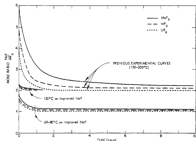
Figure 2.—Comparisons of \text{MF}_6 sorptions by previous and new techniques to obtain \text{MF}_6 \cdot 2\text{NaF} and completion of sorption to obtain \text{MF}_6 \cdot \text{NaF} .
