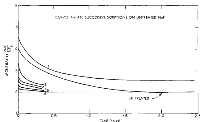
Figure 1.—Sorption of \text{UF}_6 on HF-treated and on untreated NaF to prepare \text{UF}_6 \cdot 2\text{NaF} .
