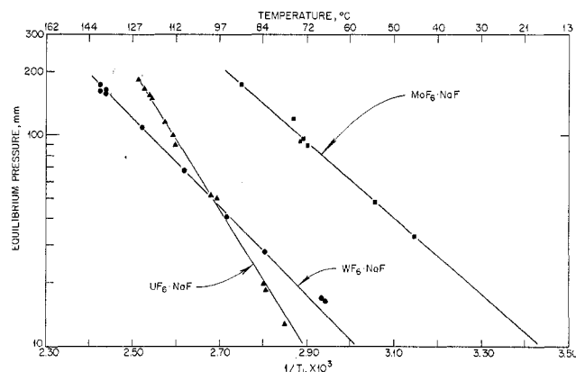
Figure 3.—Equilibrium pressures of \text{MF}_6 over \text{MF}_6 \cdot 2\text{NaF} – \text{MF}_6 \cdot \text{NaF} .
