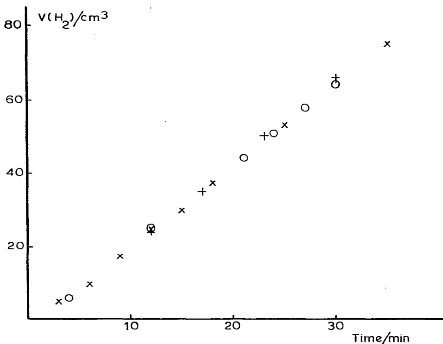
Fig. 1. Rate of evolution of \text{H}_2 in the \text{HSi}(\text{OEt})_3/\text{EtOH} reaction catalysed by [\text{IrCl}(\text{C}_8\text{H}_{14})_2]_2/4 \text{ PPh}_3 . Concentrations are: catalyst, 0.0145 M; \text{HSi}(\text{OEt})_3 , 0.172 M; \text{EtOH} , x 0.344 M, o 0.860 M, + 1.72 M. Total volume of solution, 6.91 \text{cm}^3 , solvent toluene. 100% reaction corresponds to 89.6 \text{cm}^3 \text{H}_2 .
