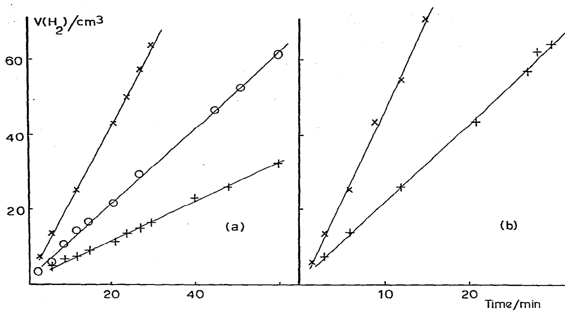
Fig. 2. Rate of evolution of \text{H}_2 in the \text{HSi}(\text{OEt})_3/\text{EtOH} reaction catalysed by \text{IrCl}(\text{N}_2)(\text{PPh}_3)_2 . Concentrations are: (a) \text{EtOH} , 0.344 M; \text{HSi}(\text{OEt})_3 , 0.172 M; catalyst, \times 0.0290 M \circ 0.0145 M + 0.00725 M. (b) \text{EtOH} , 0.344 M; catalyst, 0.0290 M; \text{HSi}(\text{OEt})_3 , \times 0.344 M + 0.172 M. Note the difference in time scales. 100% reaction corresponds to 89.6 \text{ cm}^3 \text{ H}_2 .
