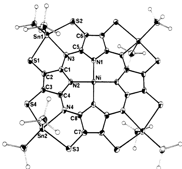
Figure 1. ORTEP diagram of 6 showing 50% probability ellipsoids. For clarity, the hydrogen atoms have been omitted and the methyl carbons have been drawn arbitrarily small.
