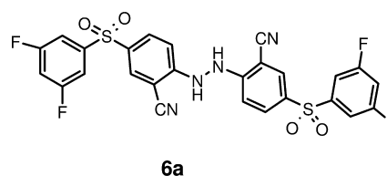
Figure 4. Dimer formation.
