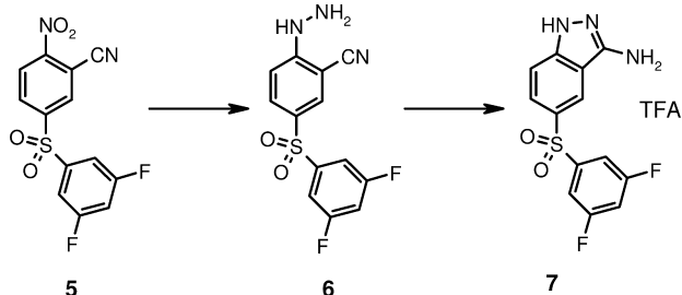
Figure 3. Possible byproducts.
