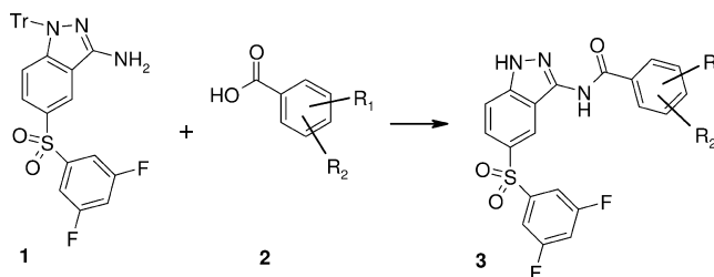
Figure 1. Subfamily compounds.
