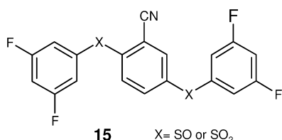
Figure 3. Possible byproducts.
