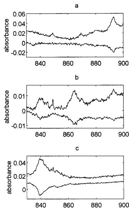
Figure 3. HOOCIO 2 : x-axis, cm -1 ; upper curves, before photolysis; lower curves, after 30 min of photolysis; the curves have been shifted for clarity. (a) (H)O—O stretch at 893.2 cm -1 in H/ 16 O 2 experiments. (b) (H)O—O stretch at 841, 865, and 893.2 cm -1 in H/ 16 O 18 O experiments. (c) (H)O—O stretch at 841 cm -1 in 18 O 2 experiments.
