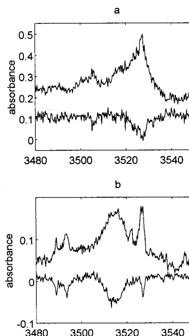
Figure 2. HOOCIO 2 : x-axis, cm -1 ; upper curves, before photolysis; lower curves, after 30 min of photolysis; the curves have been shifted vertically for clarity. (a) H— 16 O stretch at 3527.5 (overlapped by HOClO, \nu(\text{HO}) , at 3527.1 cm -1 ) and 3505.6 cm -1 . (b) H— 18 O stretch at 3514.4 and 3493.4 cm -1 . Note the difference in the photolysis rate of the broad band near 3527 cm -1 in panel a (HOOCIO 2 + HOClO) and the band at 3527.5 cm -1 in panel b (HOClO).
