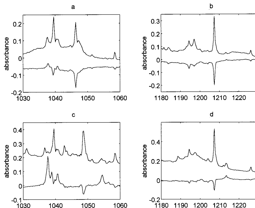
Figure 4. \text{HOOCLO}_2 : x-axis, \text{cm}^{-1} ; upper curves, before photolysis; lower curves, after 30 min of photolysis; the curves have been shifted for clarity. (a) Symmetric ClO stretch at 1046.4\text{ cm}^{-1} (with a ^{37}\text{Cl} isotope satellite at 1039.7\text{ cm}^{-1} , overlapped by \text{O}_3\nu_{\text{as}} at 1039.6\text{ cm}^{-1} ) in \text{H}/^{16}\text{O} experiments. (b) Antisymmetric ClO stretch at 1207.4\text{ cm}^{-1} (with a ^{37}\text{Cl} isotope component at 1194.4\text{ cm}^{-1} ) in \text{H}/^{16}\text{O}_2 experiments. (c) Symmetric ClO stretch at 1048.3\text{ cm}^{-1} ( ^{37}\text{Cl} isotope shift not observed) in \text{D}/^{16}\text{O}_2 experiments. (d) Antisymmetric ClO stretch at 1207.4\text{ cm}^{-1} (with a ^{37}\text{Cl} satellite at 1194.4\text{ cm}^{-1} ) in \text{D}/^{16}\text{O}_2 experiments. Note the agreement in panels a and b (taken from the same experiment) and in panels c and d (taken from the same experiment) of the photolysis rates of the ClO stretches.
