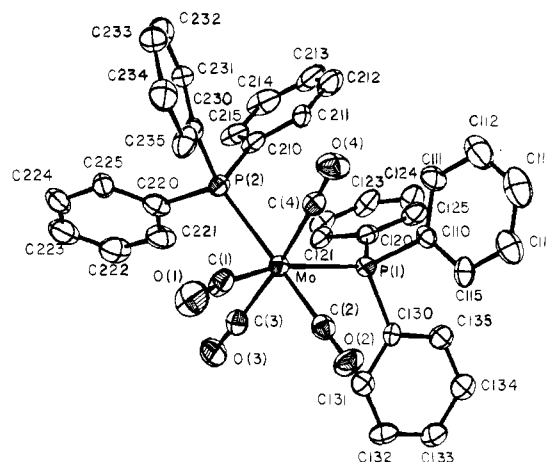
Figure 3. ORTEP drawing of the cis -Mo(CO) 4 (PPh 3 ) 2 molecule.
