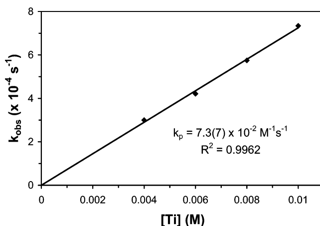
Figure 4. Plot of k_{\text{obs}} vs [\text{Ti}] of 1-hexene (1.0 M) polymerization at -10 °C using complex 9 at concentrations of 4.0, 6.0, 8.0, and 10.0 \text{ mM} at 0 °C in toluene- d_8 .
