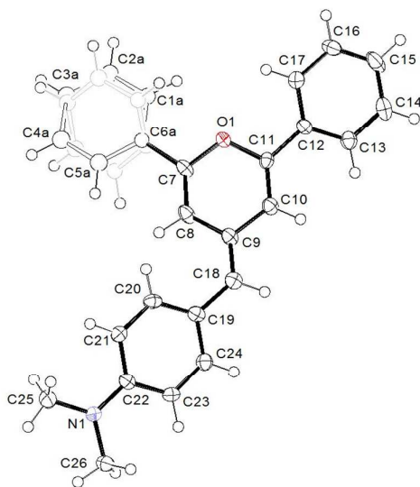
Figure 1. Molecular structure of NMe2 PhMP ( 2b ) with the atom numbering scheme. Thermal ellipsoids are drawn at 50% probability. One phenyl group is modelled as split into two positions (high thermal motion).
