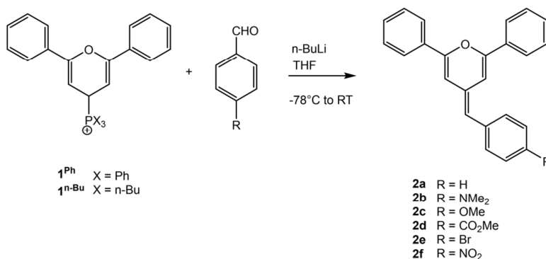
Scheme 2. Schematic pathway for the syntheses of R-substituted phenylmethylenepyran compounds 2a-f .
