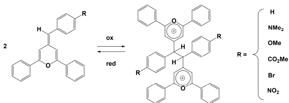
Scheme 1. Reversible C–C bond making/breaking by electrochemical oxidation of R-substituted phenylmethylenepyran ( ^R\text{PhMP} ) and reduction of their bispyrylium derivatives.
