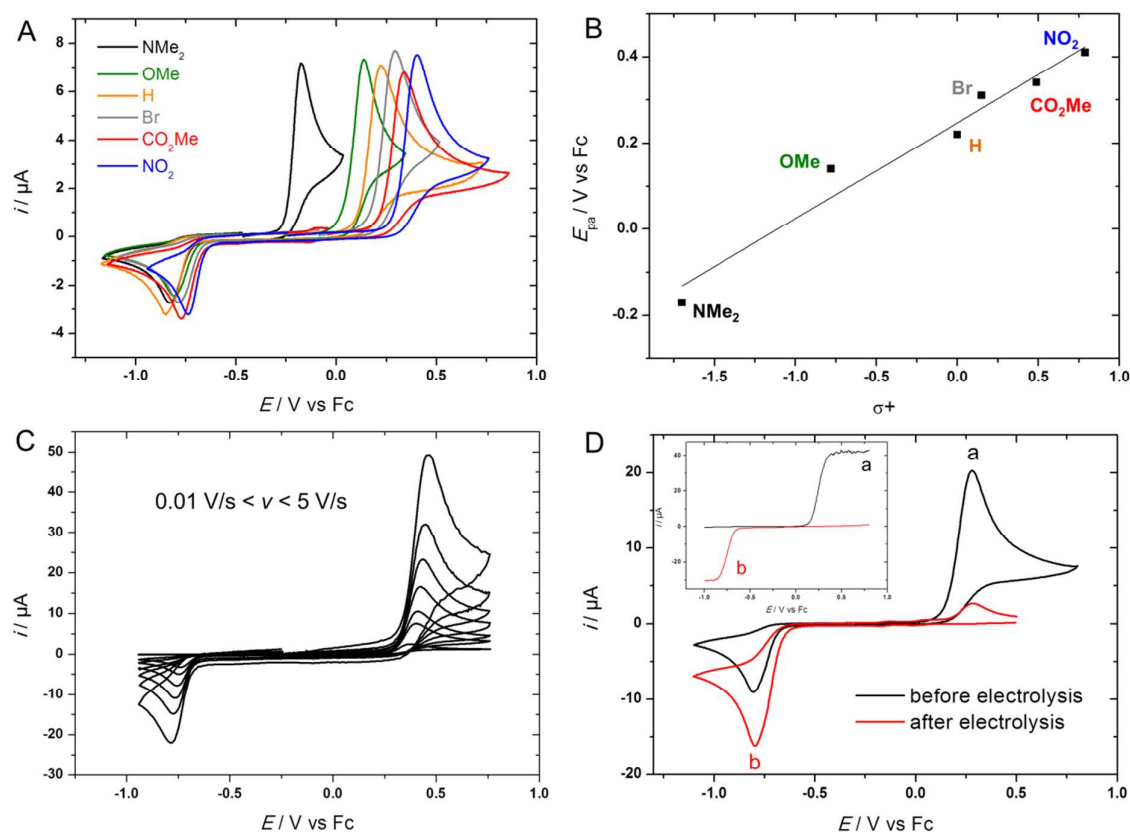
Figure 2. A) CVs at a Pt electrode of R-substituted phenylmethylenepyran compounds ^RPhMP 2a-f (0.50 mM) in CH_2Cl_2/NBu_4PF_6 0.1 M: v=0.1 \text{ V s}^{-1} ; R= NO_2 (blue), CO_2Me (red), Br (gray), H (orange), OMe (green), NMe_2 (black); B) Corresponding plots of E_{pa} vs. Brown constant \sigma^+ ; C) CVs of ^{NO_2}PhMP 2f (C=0.50 mM) for 0.01 \text{ V s}^{-1} < v < 5 \text{ V s}^{-1} ; D) CVs and RDEVs (inset) of ^HPhMP 2a (C = 1.1 mM) before (black, a) and after (red, b) exhaustive electrolysis at 0.4 V.
