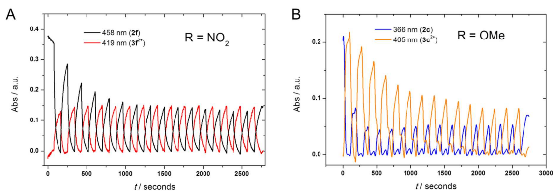
Figure 7. Plots of baseline -corrected absorbance vs time at different wavelengths starting from solutions of compounds 2f (A) and 2c (B) upon redox switching between 0.6 V and -0.9 V vs. Fc (15 cycles of 180 seconds): A) \lambda = 458 nm (black, characterizing 2f ) and 419 nm (red, characterizing 3f 2+ ); B) \lambda = 366 nm (blue, characterizing 2c ) and 405 nm (orange, characterizing 3c 2+ ). Experiments performed in CH 2 Cl 2 /NBu 4 PF 6 0.1 M with concentration of 0.60 mM in methylenepyran (optical path 0.2 mm).
