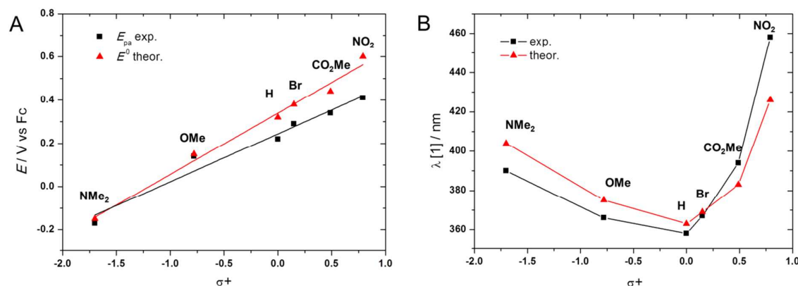
Figure 4. Plots of experimental (black squares) and calculated (red triangles) values of A) the oxidation potential in CH_2Cl_2/NBu_4PF_6 and B) the maximal wavelength \lambda[1] in CH_2Cl_2 of R PhMP 2a-f compounds against the Brown constant value of the R groups.
