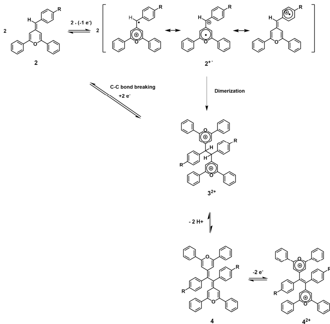
Scheme 4. Schematic pathways for the C–C bond making/breaking of R-substituted phenylmethylenepyran
