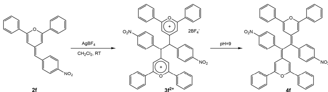
Scheme 3. Schematic pathway for the synthesis of compound 3f 2+ and 4f .
