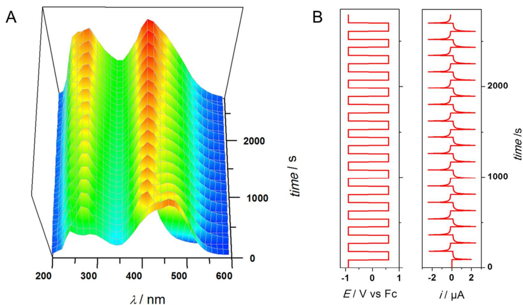
Figure 6. A) Time-resolved monitoring of the UV-Vis characterization of compound 2f in CH_2Cl_2/NBu_4PF_6 0.1 M upon redox switching between 0.6 V and -0.9 V vs. Fc (15 cycles of 180 seconds) (optical path: 0.2 mm). B) Plots of applied potential (left) and resulting current (right) against time during the monitoring.
