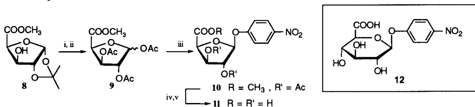
Scheme 2 Reagents and conditions : i, pyridine, \text{Ac}_2\text{O} ; ii, \text{H}_2\text{SO}_4 , \text{Ac}_2\text{O} , \text{AcOH} , 0°C; iii, \text{SnCl}_4 , \text{HO-C}_6\text{H}_4\text{-NO}_2 ; iv, \text{NaOCH}_3 , \text{CH}_3\text{OH} ; v, \text{NaOH} , \text{CH}_3\text{OH} , \text{H}_2\text{O} , 0°C.
