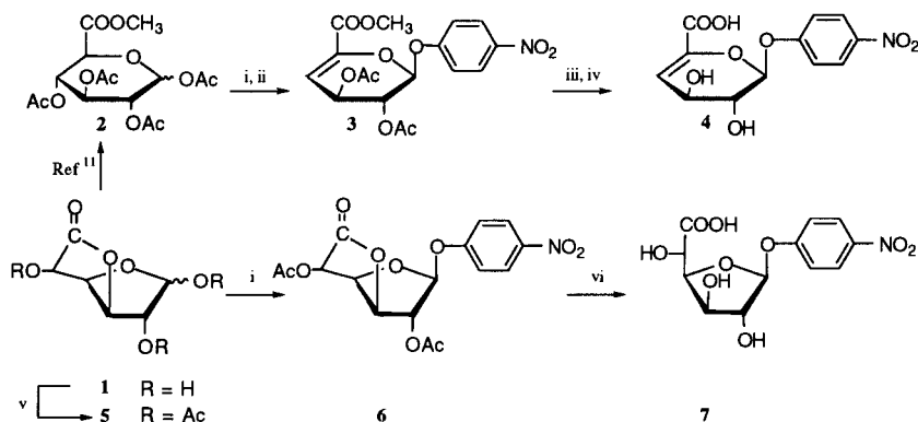
Scheme 1 Reagents and conditions : i, \text{SnCl}_4 , \text{HO-C}_6\text{H}_4\text{-NO}_2 ; ii, DBU, THF; iii, \text{NaOCH}_3 , \text{CH}_3\text{OH} ; iv, \text{NaOH} , \text{CH}_3\text{OH} ; v, pyridine, \text{Ac}_2\text{O} ; vi, (\text{CH}_3)_3\text{COK} , acetone.
