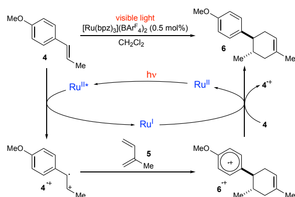
Scheme 1. Proposed Photocatalytic Radical Cation Diels–Alder Cycloaddition Mechanism
