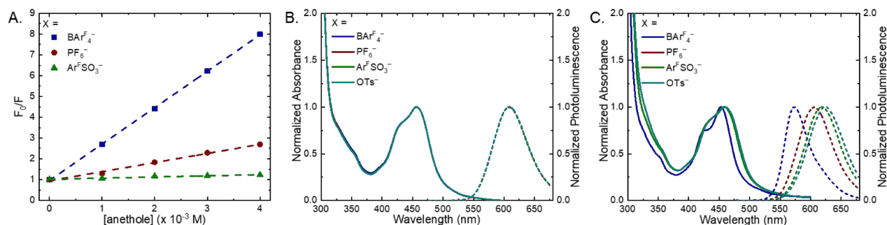
Figure 2. A. Stern–Volmer plots for excited-state quenching of catalysts 3a – c in \text{CH}_2\text{Cl}_2 . B/C. Effect of counteranion identity on excited-state properties of [\text{Ru}(\text{btfmb})_3](X)_2 , X is indicated in the legend. (B) Absorption (solid line) and photoluminescence (dashed line) spectra in MeCN. (C) Absorption (solid line) and photoluminescence (dashed line) spectra in \text{CH}_2\text{Cl}_2 .
