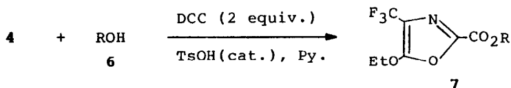
Scheme 2.
